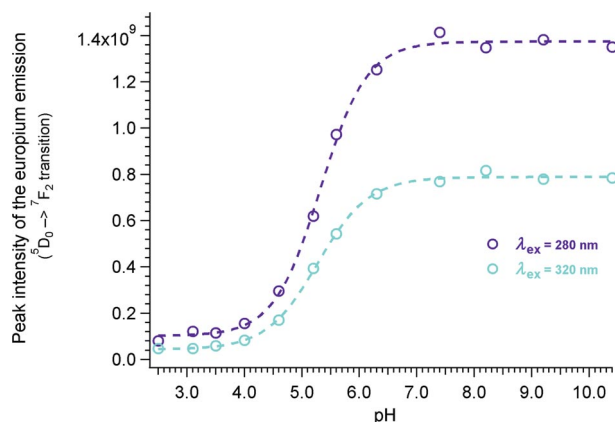
Figure 4. Peak intensity of the [\text{Eu}(\text{DPApC})_3]^{3-} ^5\text{D}_0 \rightarrow ^7\text{F}_2 transition in aqueous solution as a function of pH.
